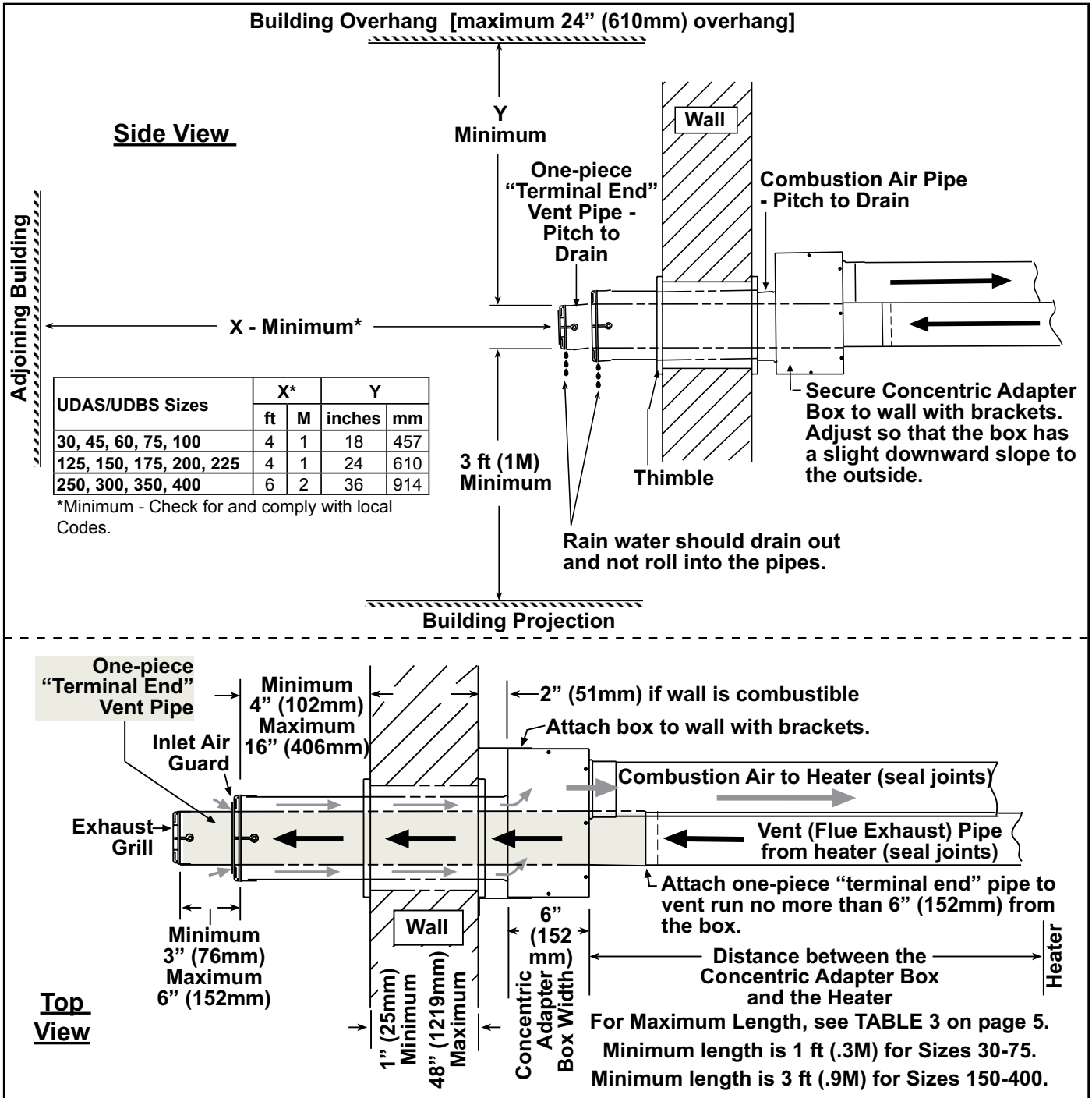
FIGURE 12 - Installation of a Typical Separated-Combustion Unit with Horizontal Vent Terminal and Combustion Air Pipe (Option CC6)
