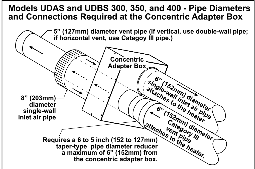
FIGURE 9 - Concentric Adapter Box Connections for Sizes 300, 350, and 400
