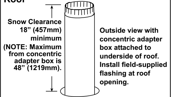
FIGURE 14 - Slide attached Combustion Air Pipe up through the Roof
