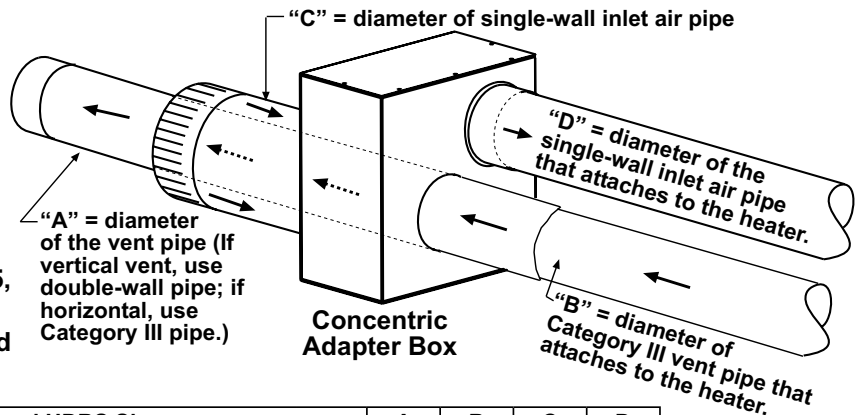
FIGURE 8 - Concentric Adapter Box Connections for Sizes 30, 45, and 60 using 4" (102mm) diameter pipes and for all of Sizes 75, 100, 125, 150, 175, 200, 225, and 250
