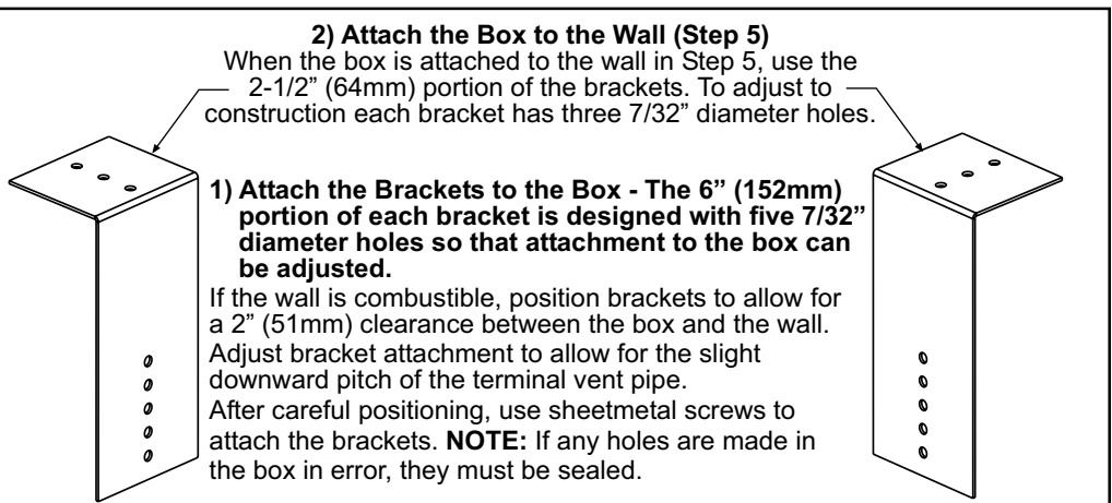
FIGURE 11 - Brackets for Attaching the Concentric Adapter Box to the Wall
