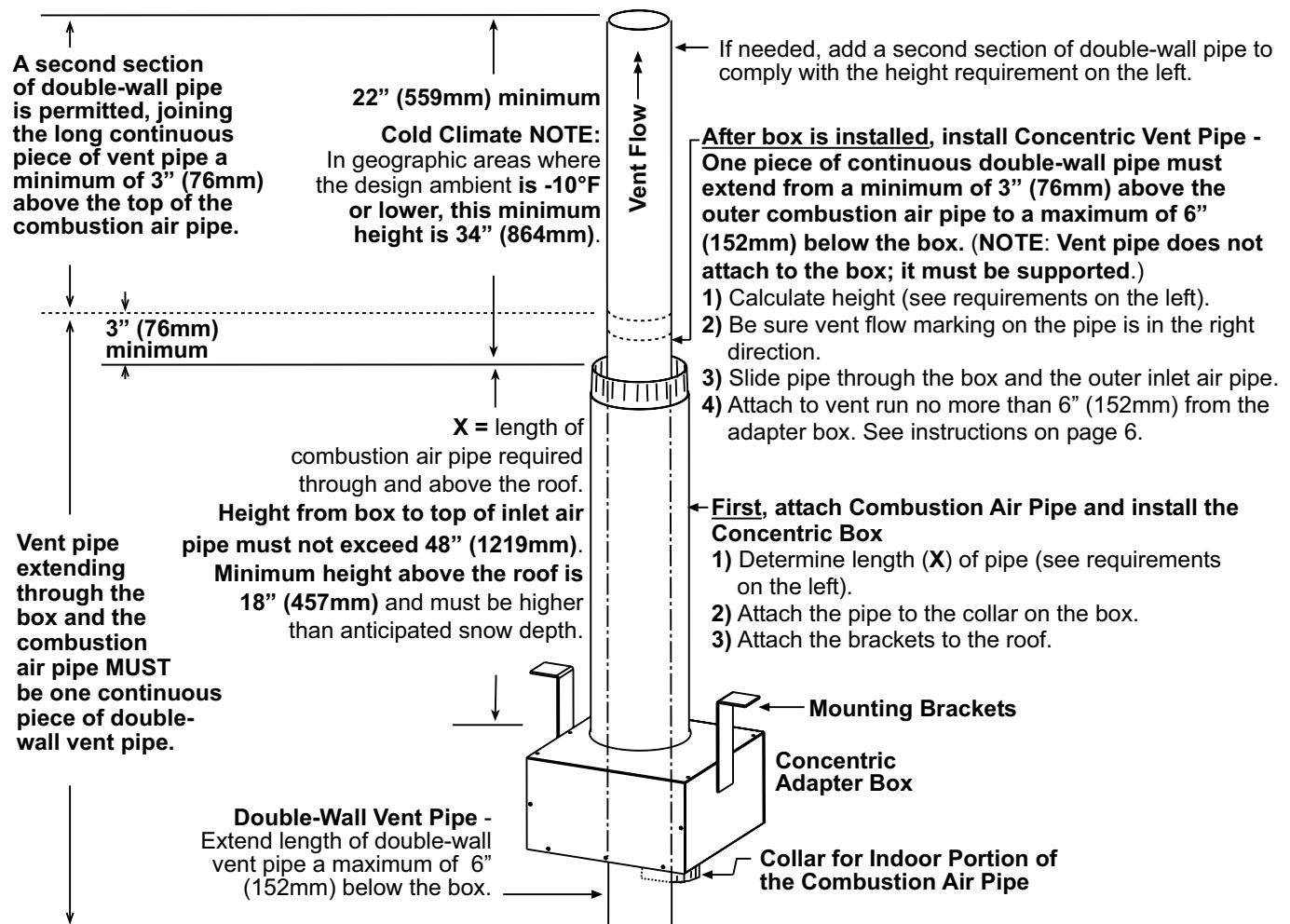
FIGURE 14 - Concentric Adapter Box, Outdoor Combustion Air Pipe, and Concentric Vent Pipe
