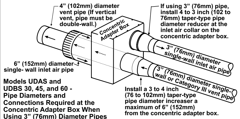
FIGURE 7 - Concentric Adapter Box Connections for Sizes 30, 45, and 60 using 3" (76mm) diameter pipes
