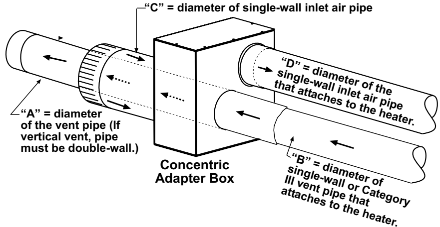
FIGURE 8 - Concentric Adapter Box Connections for Sizes 30, 45, and 60 using 4" (102mm) diameter pipes and for all Installations of Sizes 75, 100, 125, 150, 175, 200, 225, and 250
