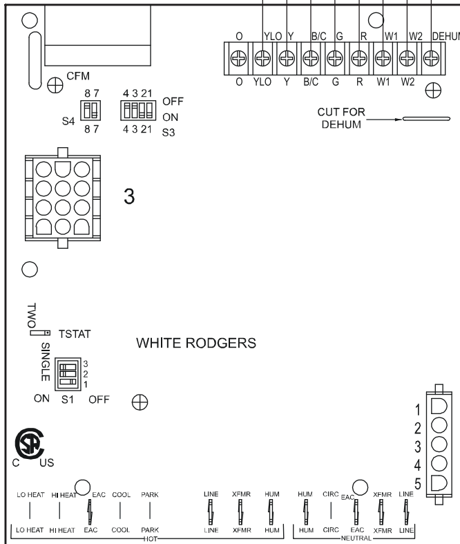
TWO-STAGE GAS FURNACE
